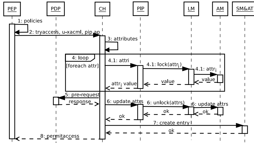
Fig. 3. Sequence Diagram for Pre-Authorization
