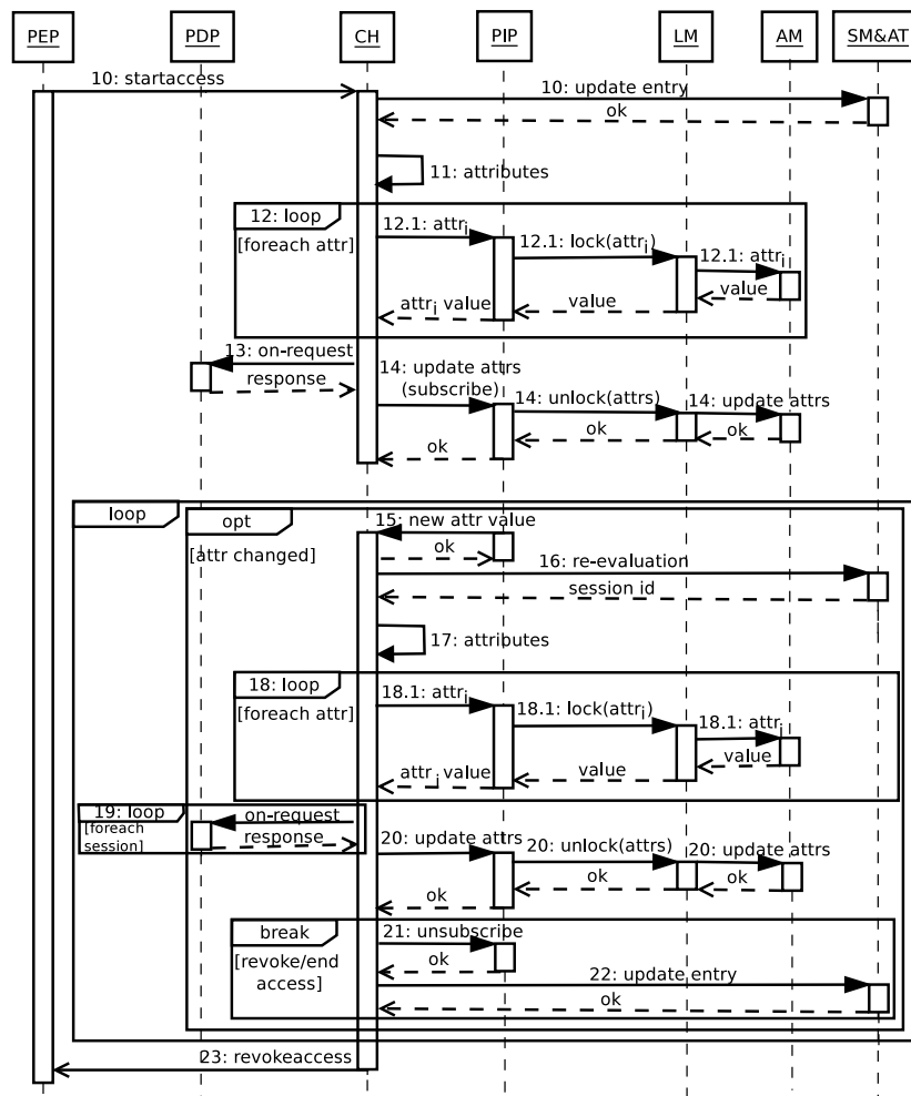
Fig. 4. Sequence Diagram for Ongoing Authorization
