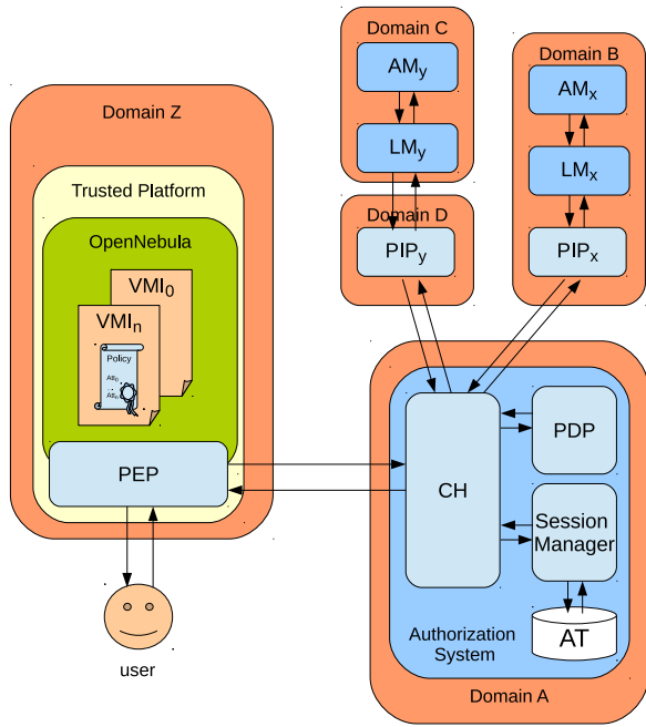
Fig. 2. Architecture for Enforcement of Data Usage Policy
